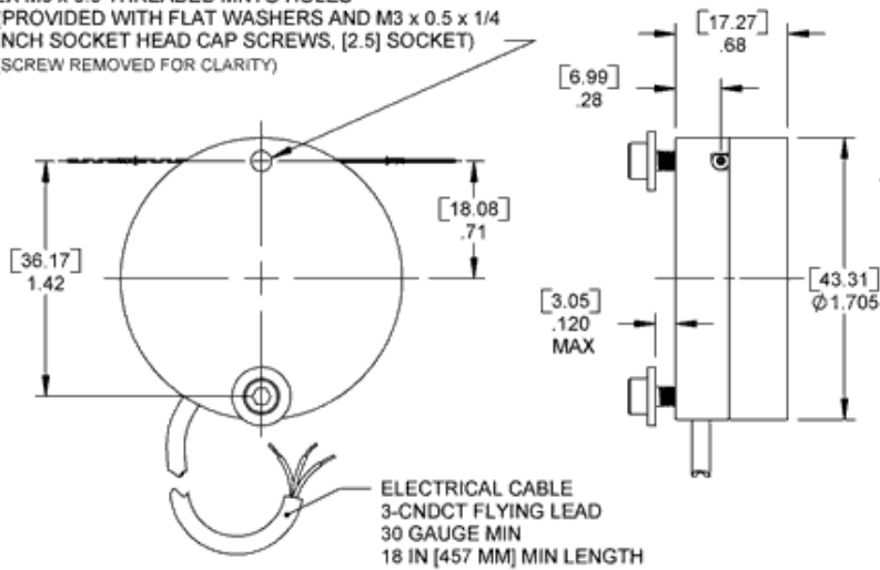
Electrical Connection for Increasing Output with Displacement Cable Extraction
